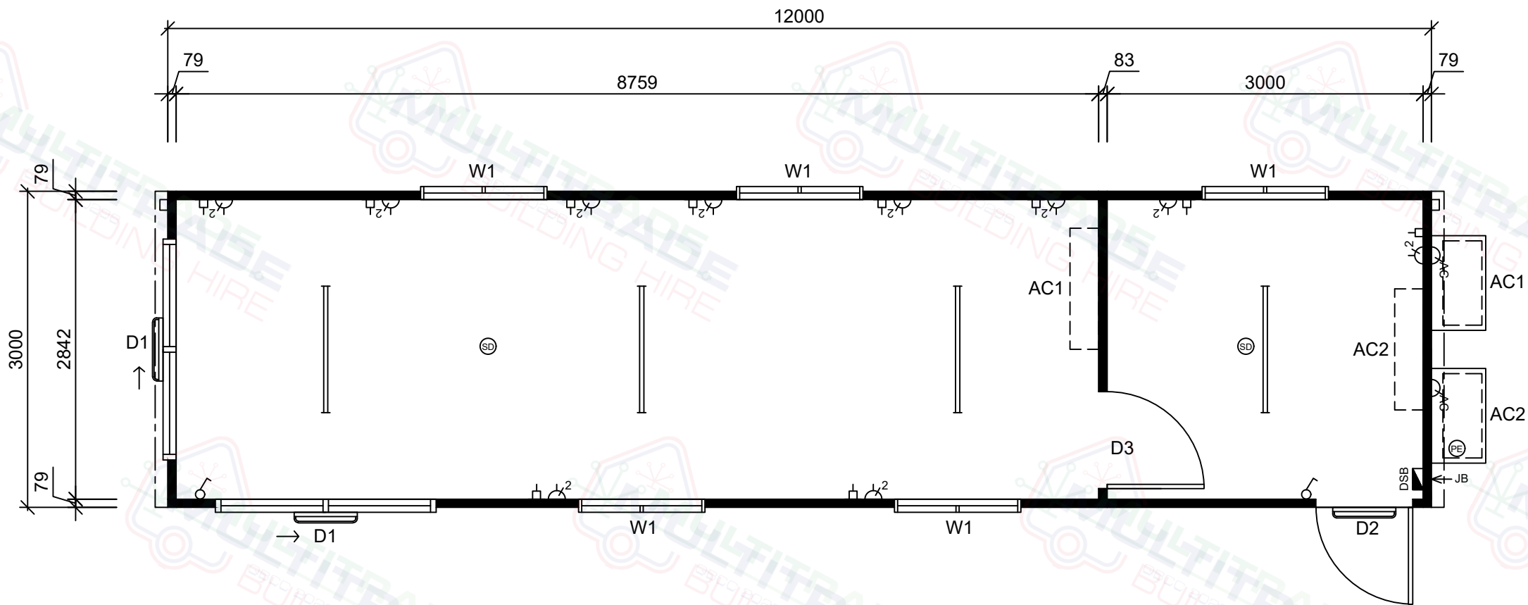
12.0x3.0m Office - Floor Plan
